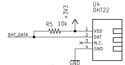
DHT22 (Digital Temp./Humidity) Monitors the ambient temperature and humidity in proximity to the sensor. Likely mounted to the board.
