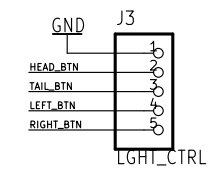
Light Control Buttons Pulling these lines to GND will toggle the corresponding lights.
