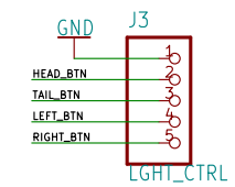
Light Control Buttons Pulling these lines to GND will toggle the corresponding lights.
