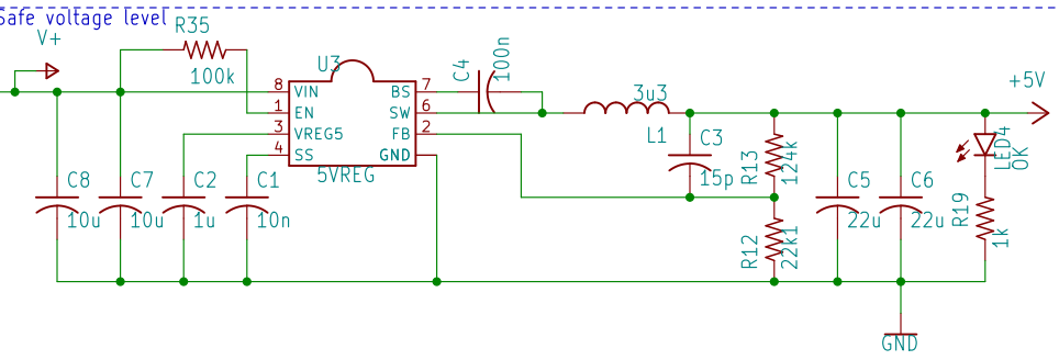
5V/4A Buck Converter Supplies power to RPI, the 3V3 comes from RPI's regulators to the system. Uses AP65450SP-13 chip and the 5V reference design in the datasheet. If there is any power fault leading up to this an appropriate LED will indicate it, otherwise the OK will light.
