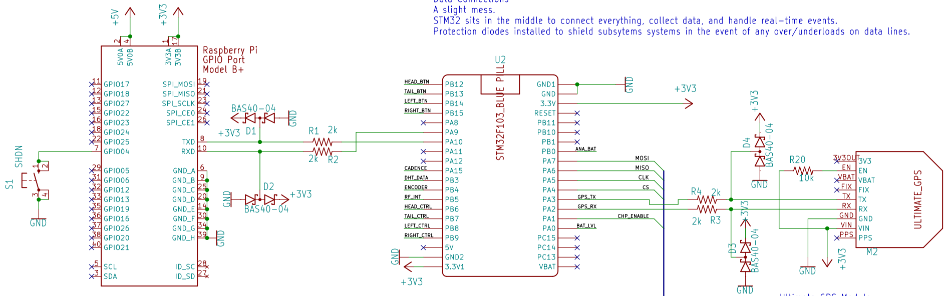
Ultimate GPS Module Used to gather GPS data, including speed as a backup for the encoder.
