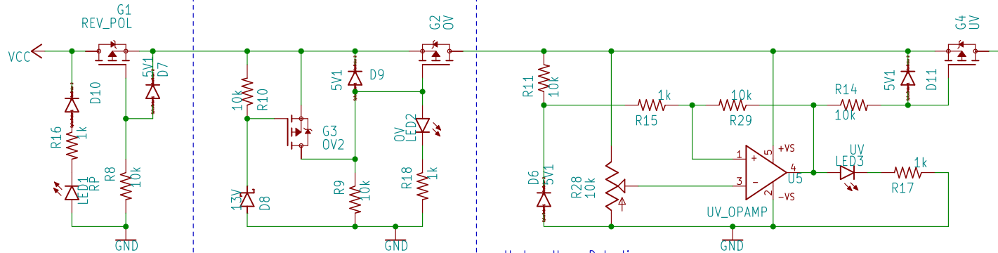
Reverse Polarity Protection First stage of protection from the battery Over Voltage Protection Kicks in based around value of D8 (Currently 13V) Undervoltage Detection Used to prevent draining batteries too far and causing cell damage. Cutoff threshold determined by the potentiometer. Hysteresis to prevent oscillating.
